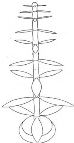
FIG. 94. — The whorled arrangement.
